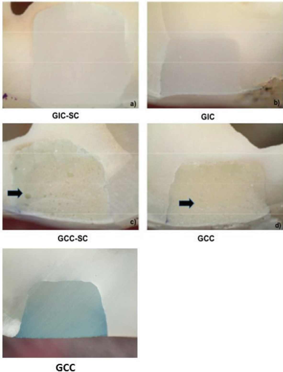
Figures 1 a-e. T Representative stereomicroscope images of specimens restored with a) GIC-SC (Score 0), b) GIC (Score 1), c) GCC-SC (Score 2), d) GCC (Score 2), e) GCC (Score 3) (x30). Note the porous surface in c and d restored with GCC without and with surface coating indicated by arrow. For group abbreviations, see Table 1.
